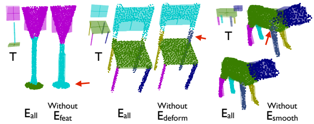
Figure 4: Energy function example. Effect of every energy term in the template fitting procedure. For all the three examples, we show a result with all the energy terms (left) and with one energy term excluded (right). (Left-to-right) The stem merges with the base if local shape features are excluded for goblets; chair legs are extended towards back support if we exclude statistical plausibility of a template deformation; and the segmentation boundary between the head and the torso of an animal is noisy in the absence of the smoothness term.
