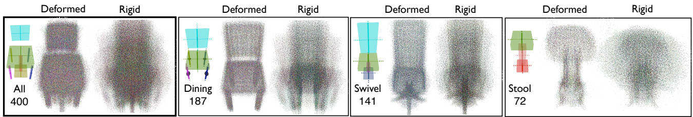
Figure 8: Co-aligned shapes. We use template deformation parameters ( r, d ) to align all shapes from the set of 400 chairs in COSEG dataset to their corresponding mean part arrangements and scales (left image). And compare it to just using rigid transformations r to co-align shapes (right image). Note that our deformation model leads much sharper co-alignments by factoring out the dominant deformation modes.
